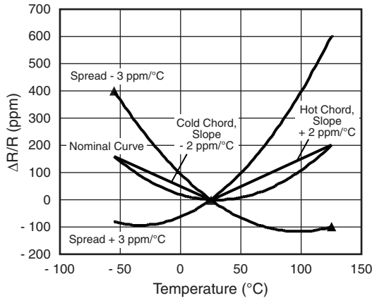
Fig. 1 - ( \Delta R/R = f(T) ) Chart of Resistors of \pm 5 ppm/ ^{\circ}\text{C} TCR
