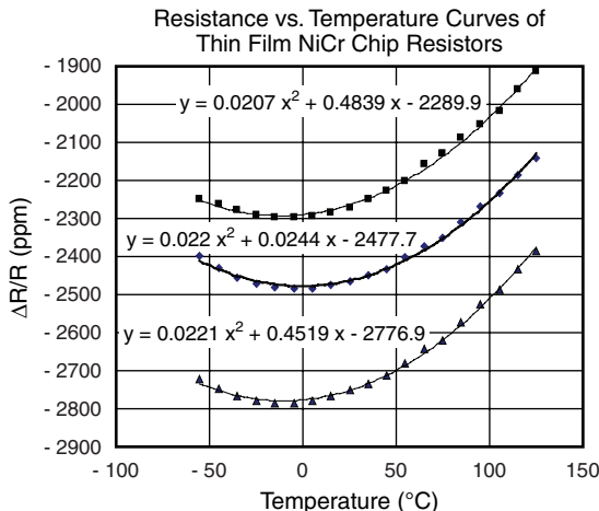
Fig. 5 - Fig. 5: Recording of \Delta R/R every 10°, Quadratic Trendlines and Equations of Three NiCr Thin Film Chips
