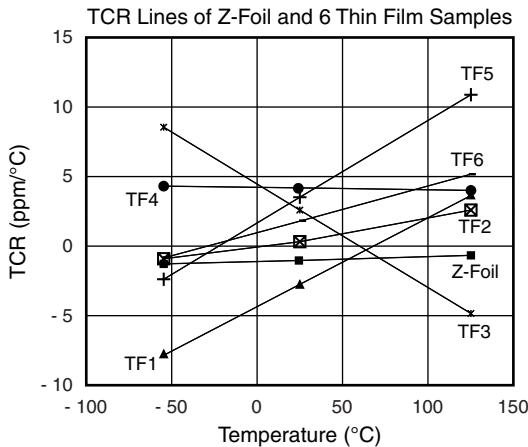
Fig. 10 - Temperature Coefficient of Resistance as Function of Temperature of Resistor Chips per Fig. 7
