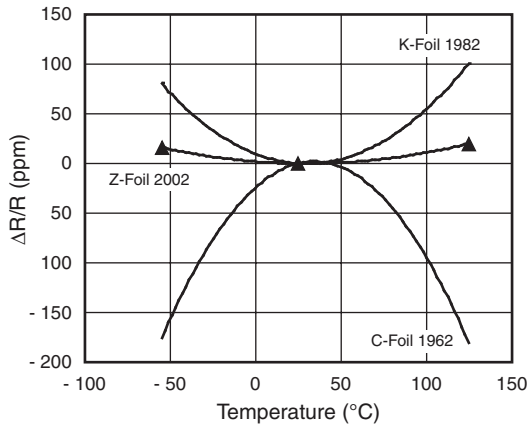
Fig. 4 - Fig. 4: Three Resistance vs. Temperature Characteristics of Foil Resistors and Year of their Introduction
