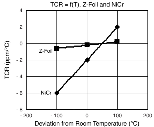
Fig. 7 - Temperature Coefficient of Resistance vs. Temperature Plot of Thin Film and Z-Foil Resistors Shown in the Fig. 6
