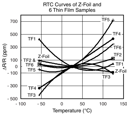
Fig. 9 - Relative Resistance Change vs. Temperature Curves of Z-foil and Thin Film Precision Chip Resistors from 6 Vendors
