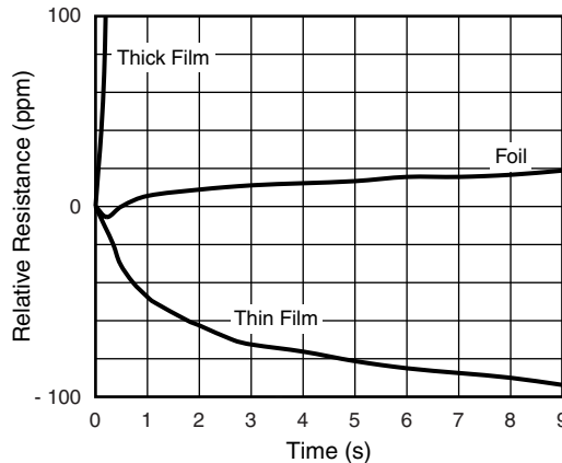
Fig. 8 - Stabilization Time of Z-Foil, Typical Thin Film and Thick Film Resistors
