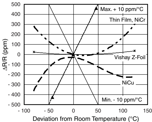
Fig. 3 - Typical \Delta R/R = f(T) Curves of Z-Foil, NiCu and NiCr (Thin Film) Resistors within the Maximum Chord Slopes of + 10 ppm/°C and - 10 ppm/°C
