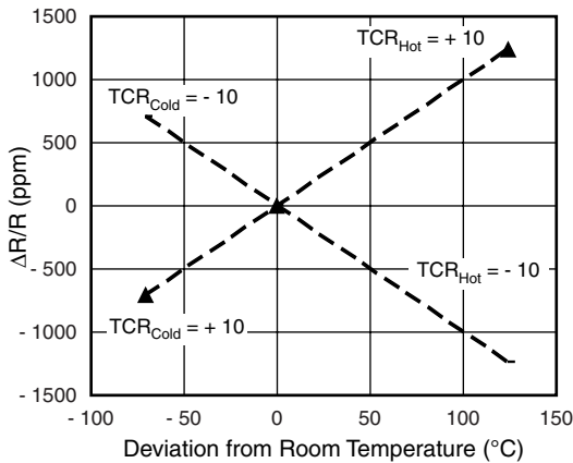
Fig. 2 - Limiting Chord Slopes for Resistors of Stability Class 0.1 Defining a TCR of 10 ppm/°C
